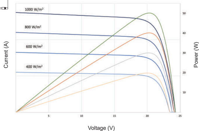
RNG-50DB-H Characteristics Versus Voltage
